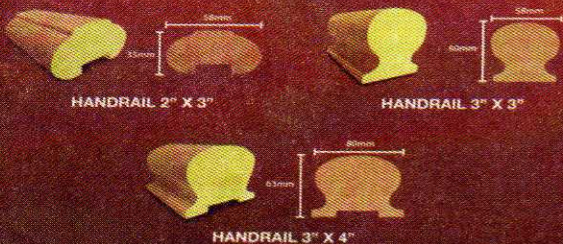
HANDRAIL 3" X 4"
